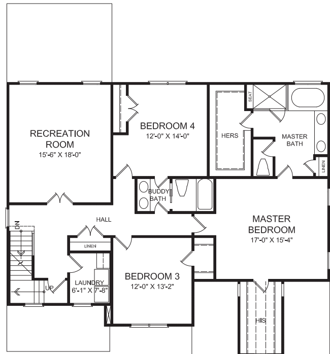
SECOND FLOOR
